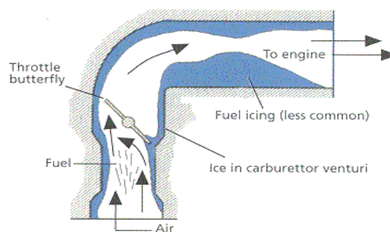
BUILD-UP OF ICING IN INDUCTION SYSTEM
